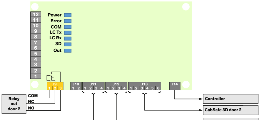
Figure 6: cegard/Smart sensor connection PCB / extension module
