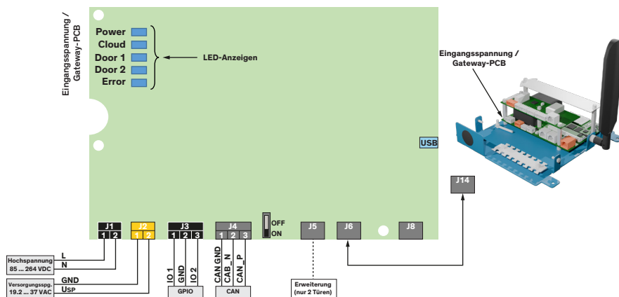
Figure 22: LED Indicators Gateway Interface PCB
