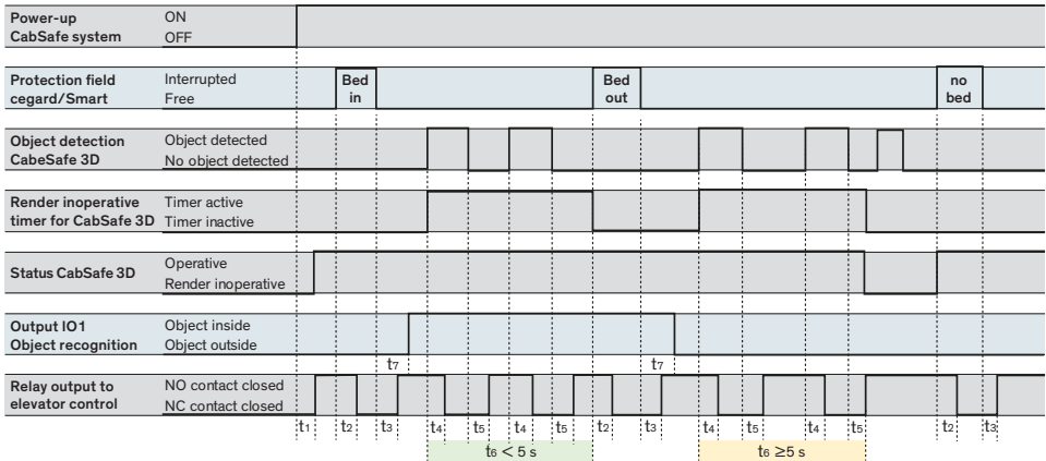
Figure 18: Timing diagram (output logic selection DIP 10 = 0)
