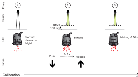
Figure 15: Configuration T type with the teach-in button
