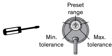
Figure 16: Tolerance adjustment (+/-) according sensor naming
