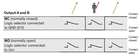
Figure 18: Logic selector
